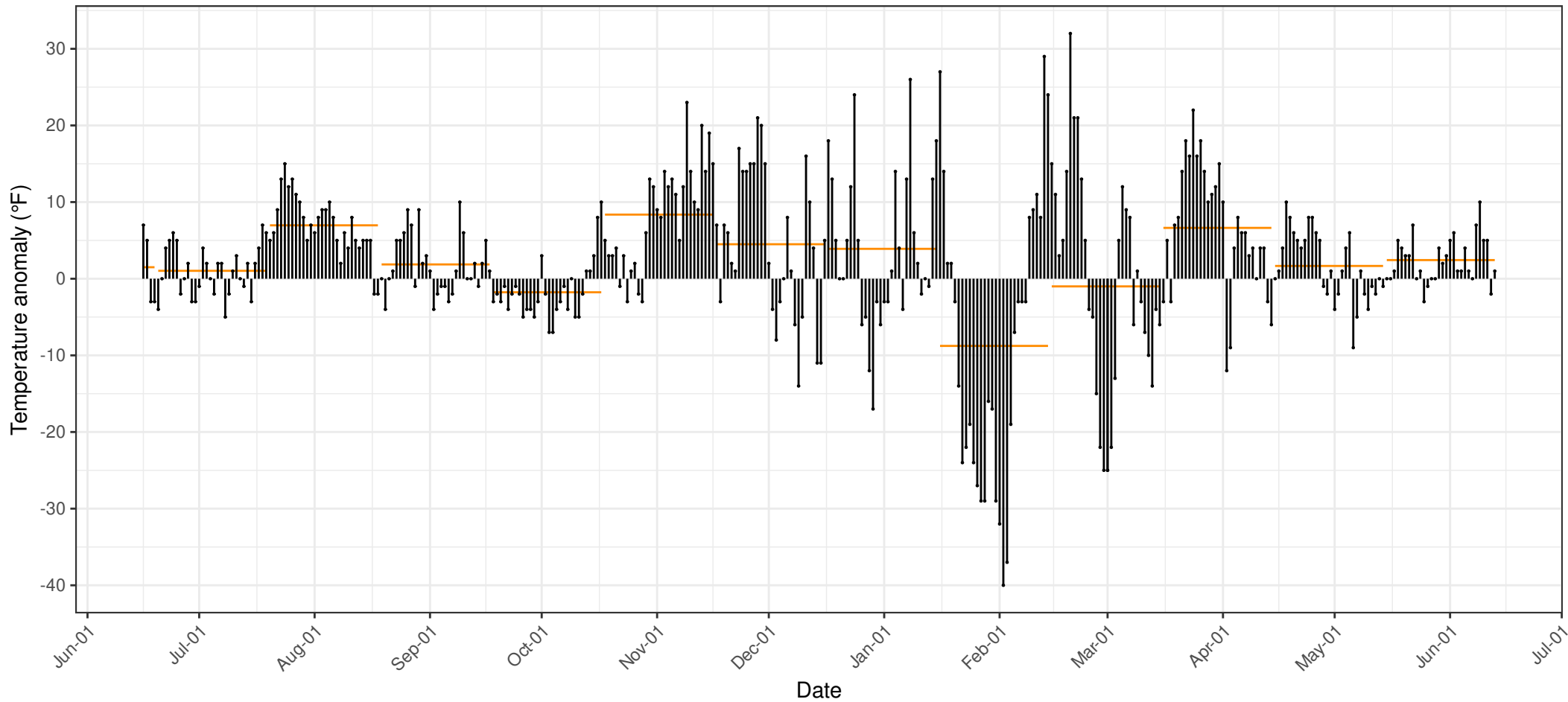
Difference between daily mean temperature and 30-year average, Fairbanks Airport (PAFA) 2023–2024
