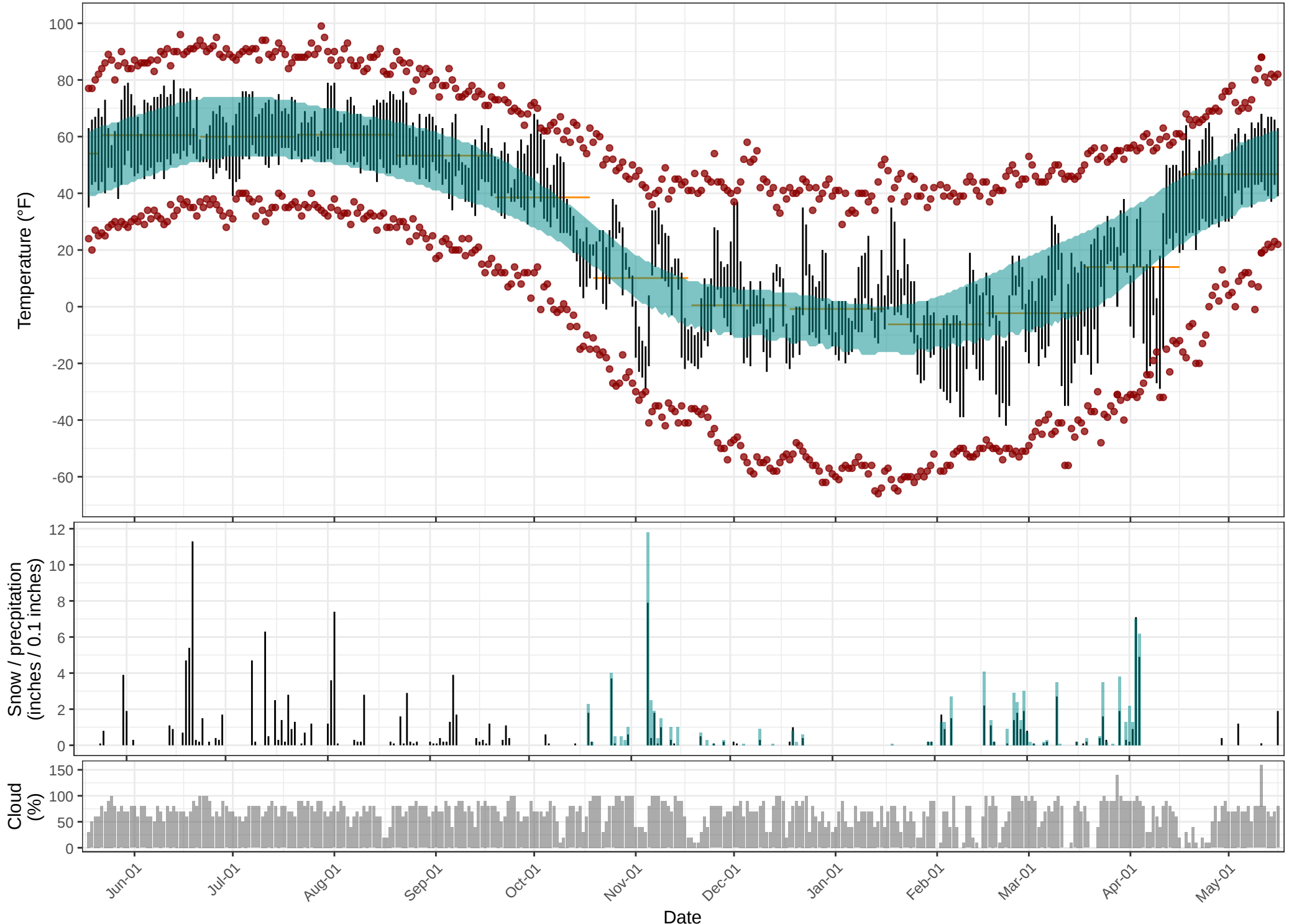
Daily temperature, precipitation and cloud cover, Fairbanks Airport (PAFA) 2020–2021
