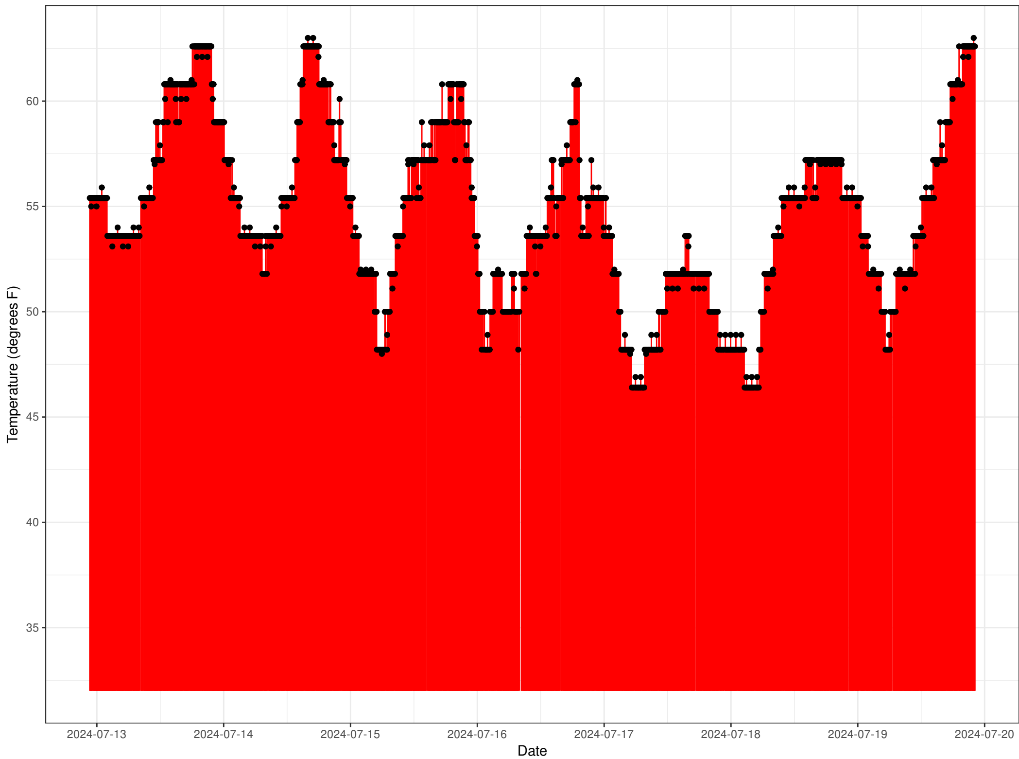
Temperature data for station PFNO
