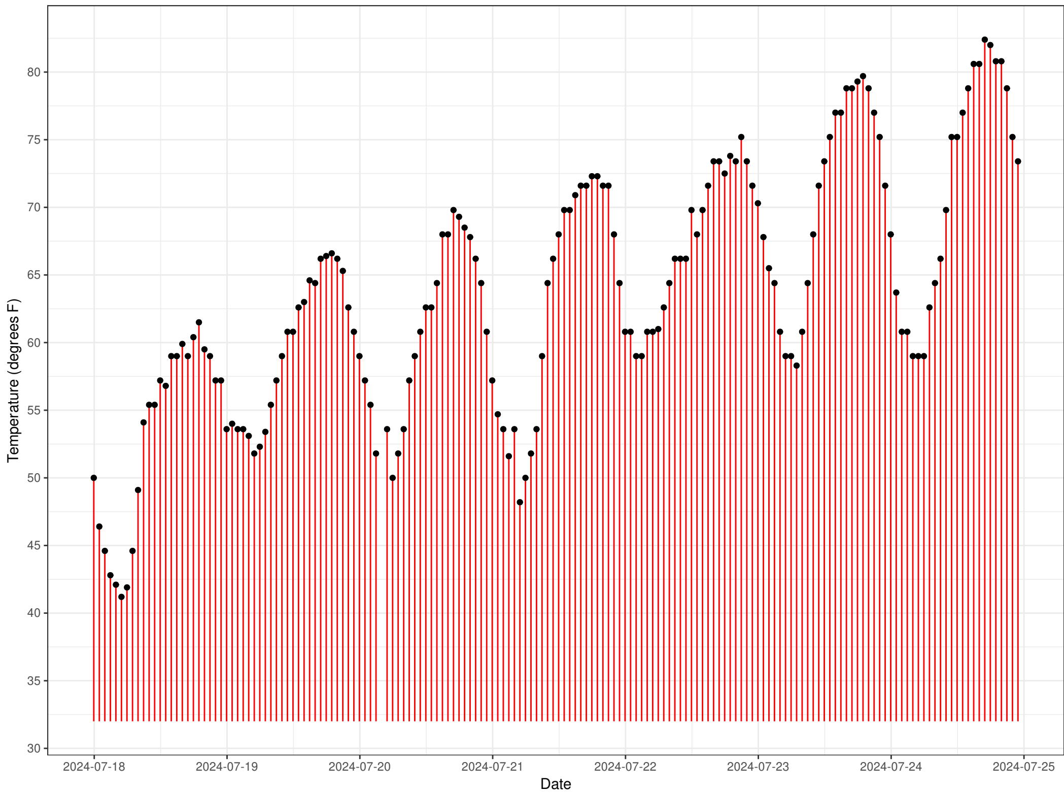
Temperature data for station PAIM
