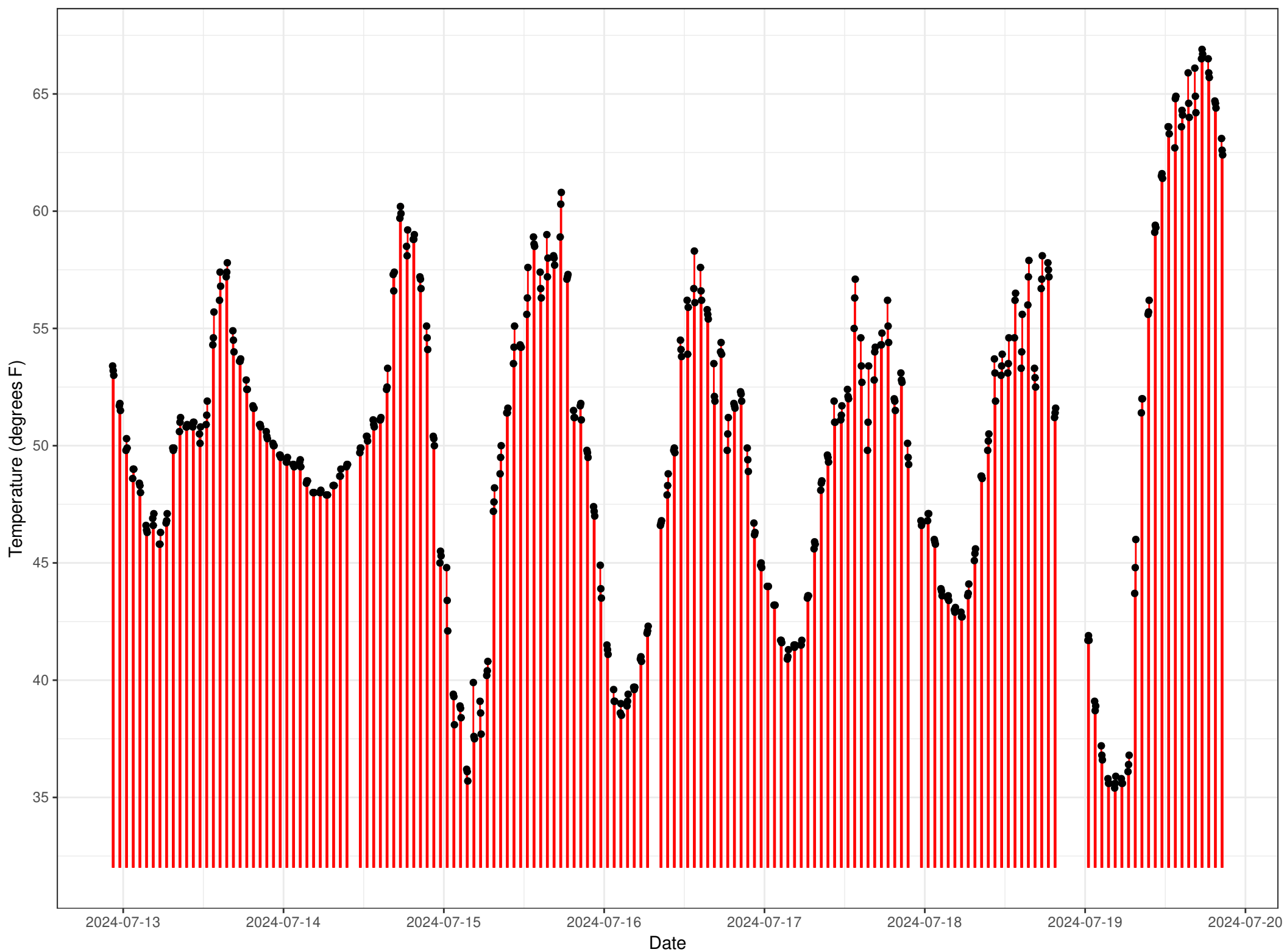
Temperature data for station GNNA2
