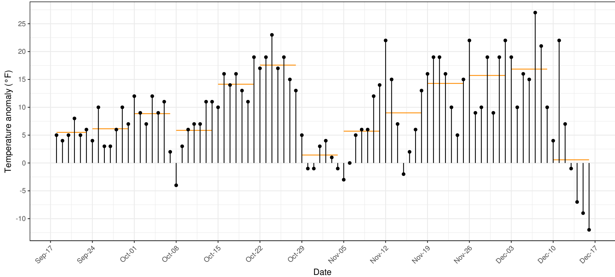
Difference between daily mean temperature and 30-year average, Fairbanks Airport (PAFA) 2018
