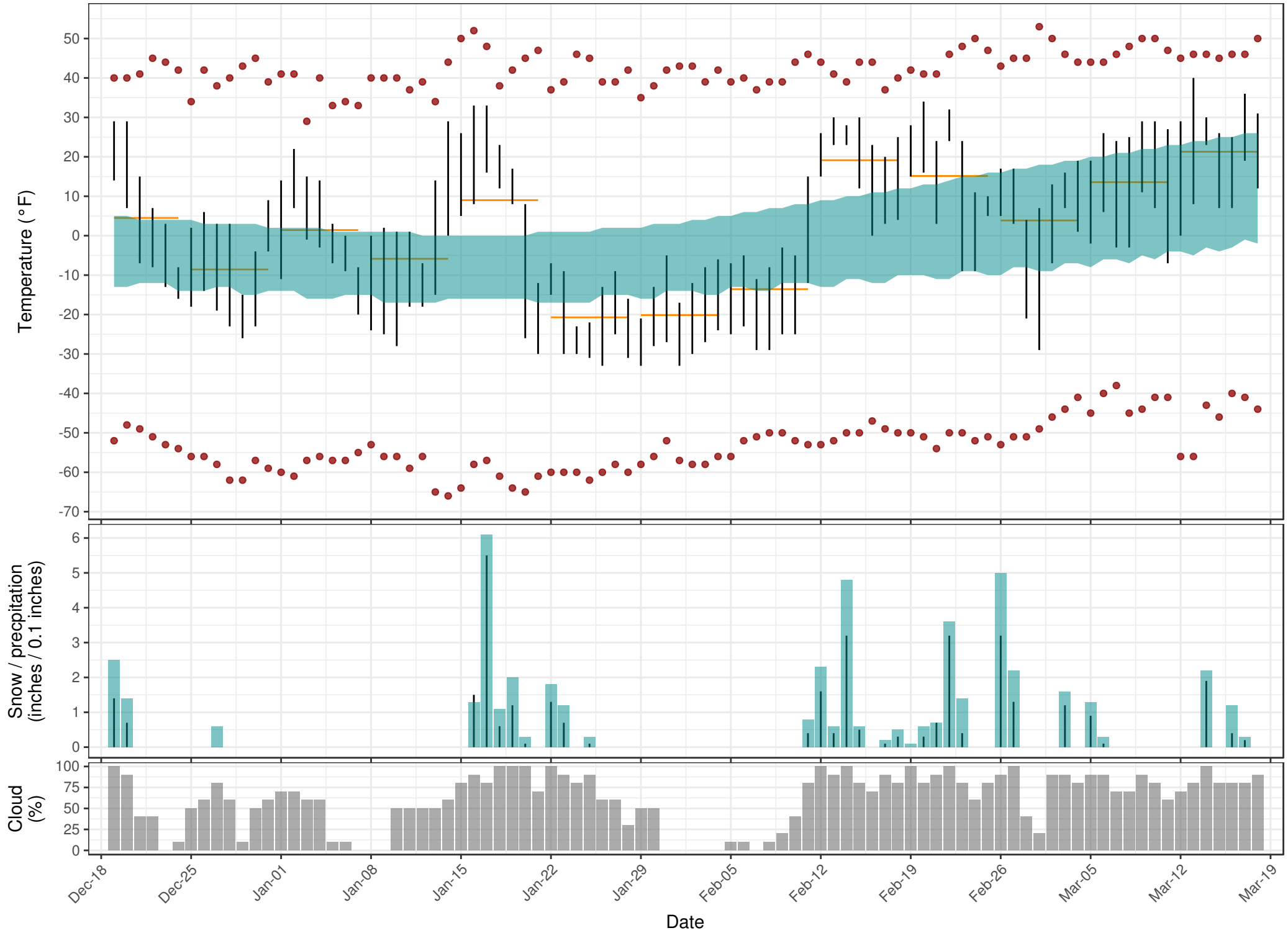
Daily temperature, precipitation and cloud cover, Fairbanks Airport (PAFA) 2017–2018
