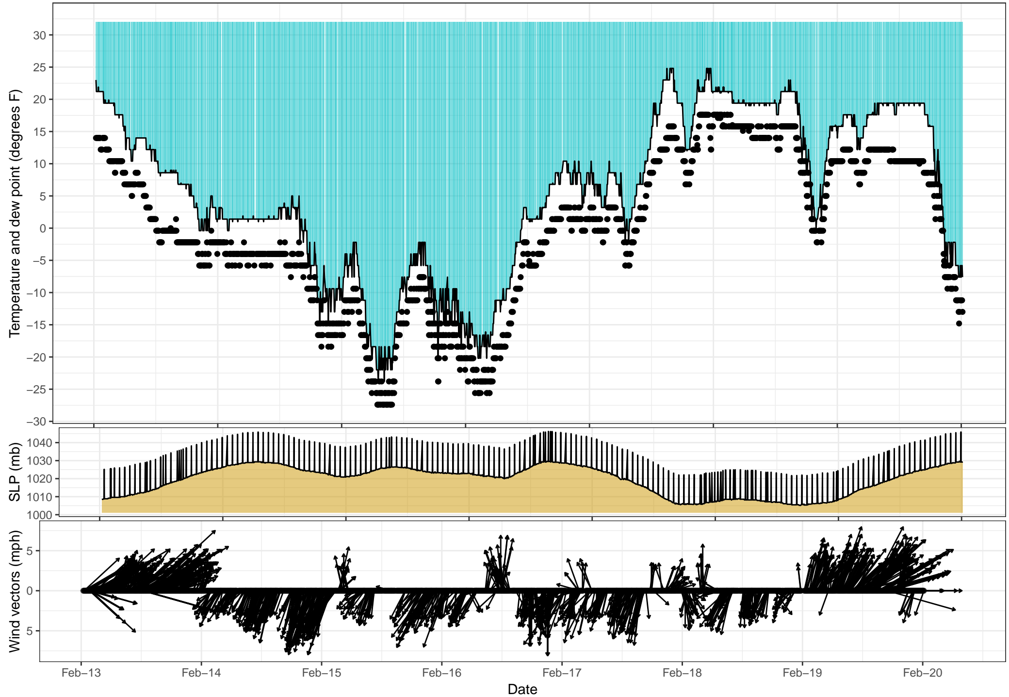
Temperature, dew point, barometric pressure and wind, Fairbanks Airport (PAFA)
